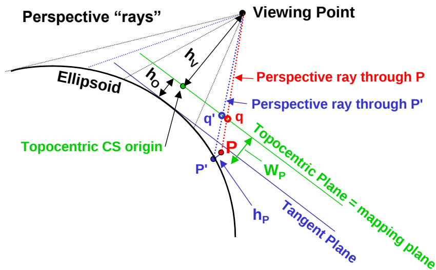
Figure 12 – Vertical perspective.
