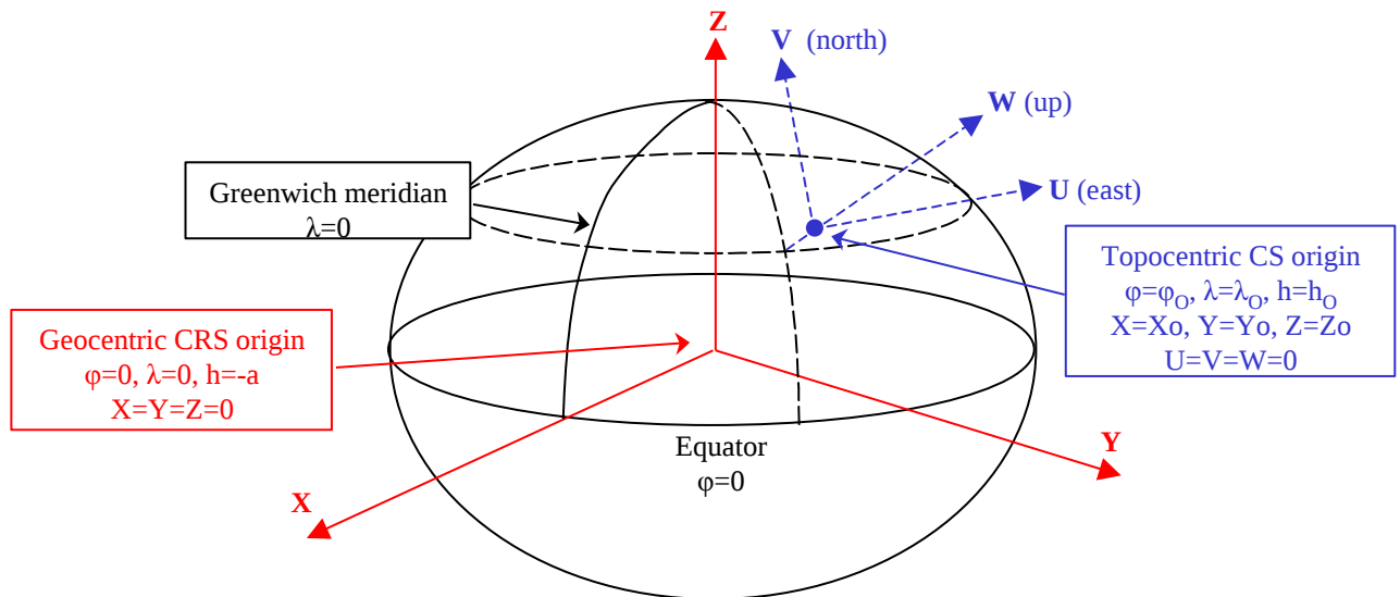
Figure 13 – Topocentric and geocentric systems.
