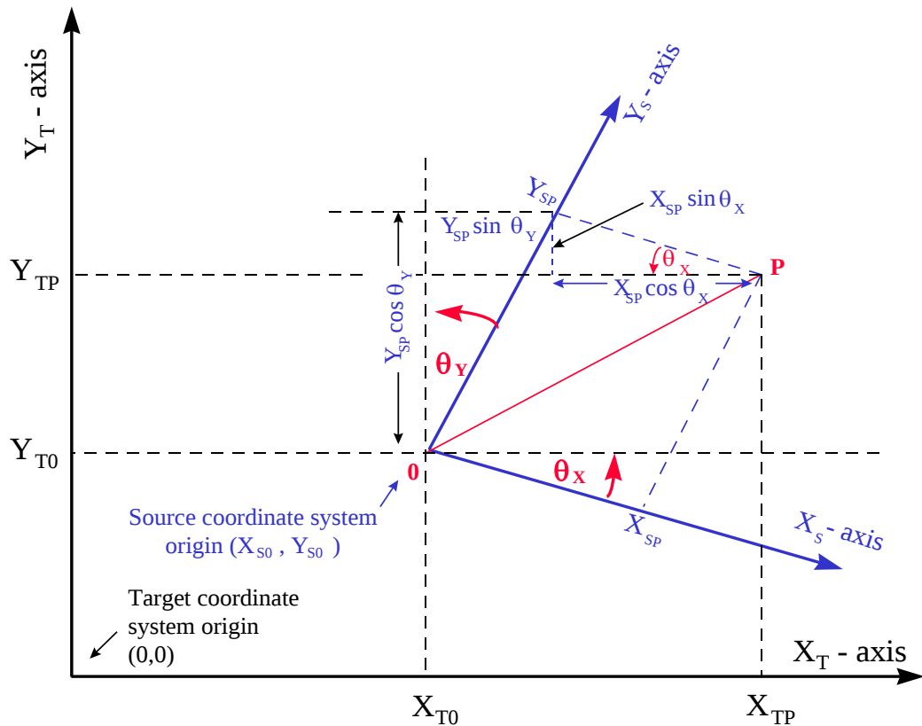
Figure 14 – Geometric representation of the affine coordinate transformation. (Note that the scale parameters of the X_S and Y_S axes have been omitted to prevent cluttering of the figure).
