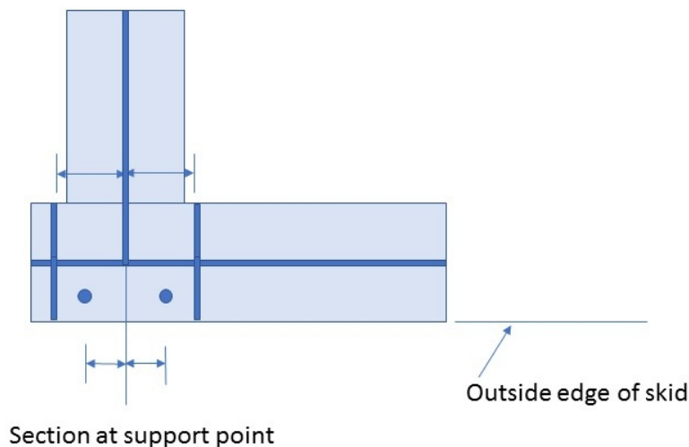
Figure 4 — Foundation for equipment \geq 1\,000 kg (2 200 lb) operational weight, section at support point showing bolt positions at support
