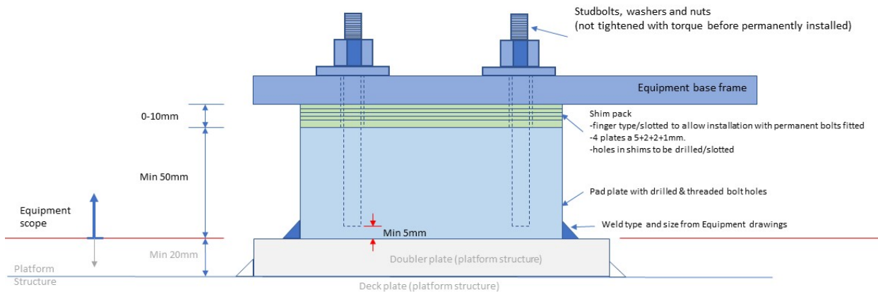
Figure 3 — Foundation for equipment \geq 1\,000 kg (2 200 lb) operational weight, interface design and responsibilities, single securing nut
