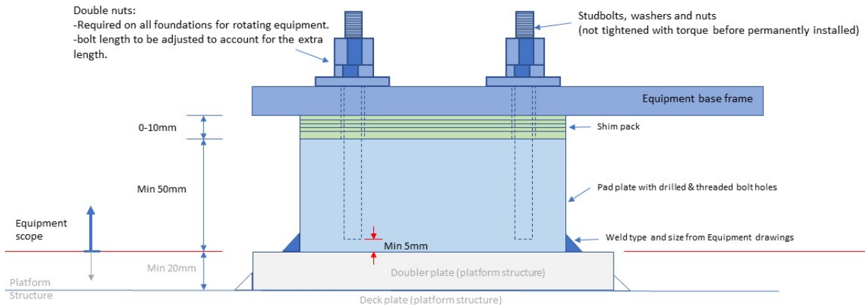
Figure 2 — Foundation for equipment \geq 1\,000 kg (2 200 lb) operational weight, interface design and responsibilities, double securing nut
